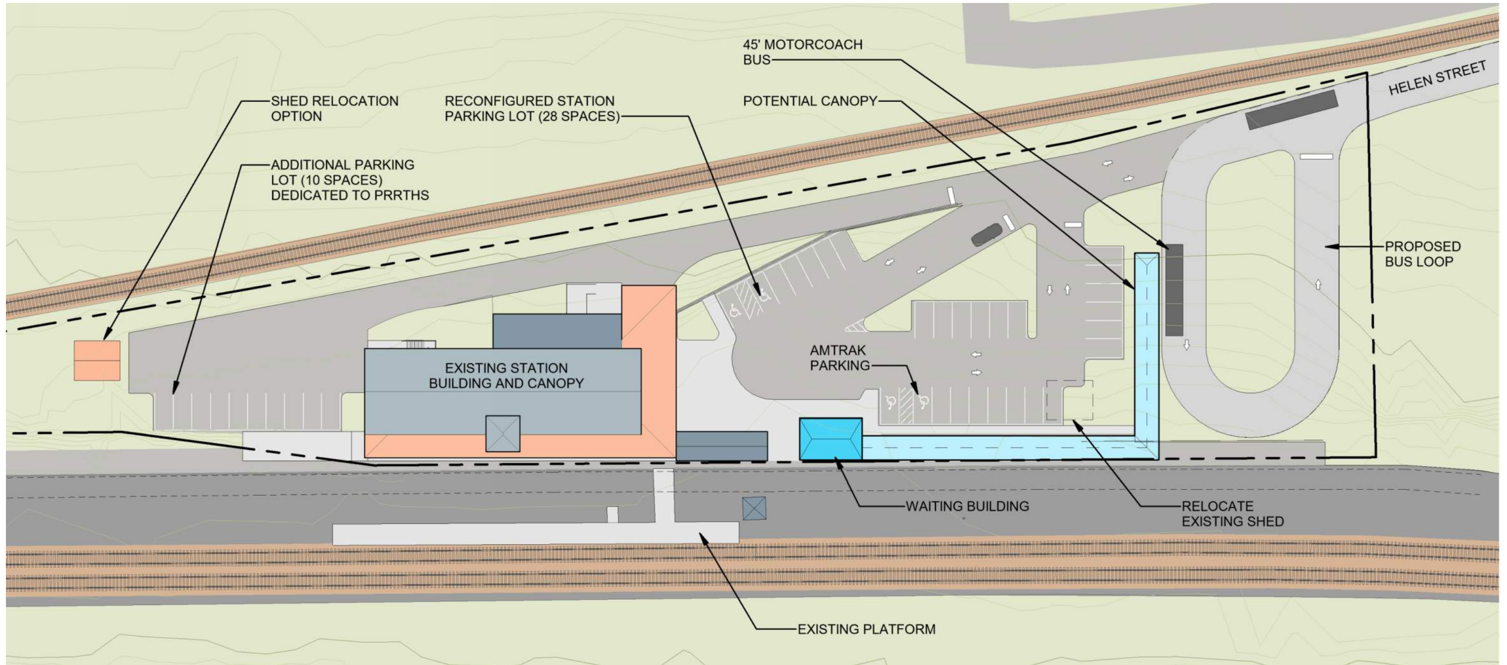
SITE PLAN OPTION 1 – WITH BUS STOP
