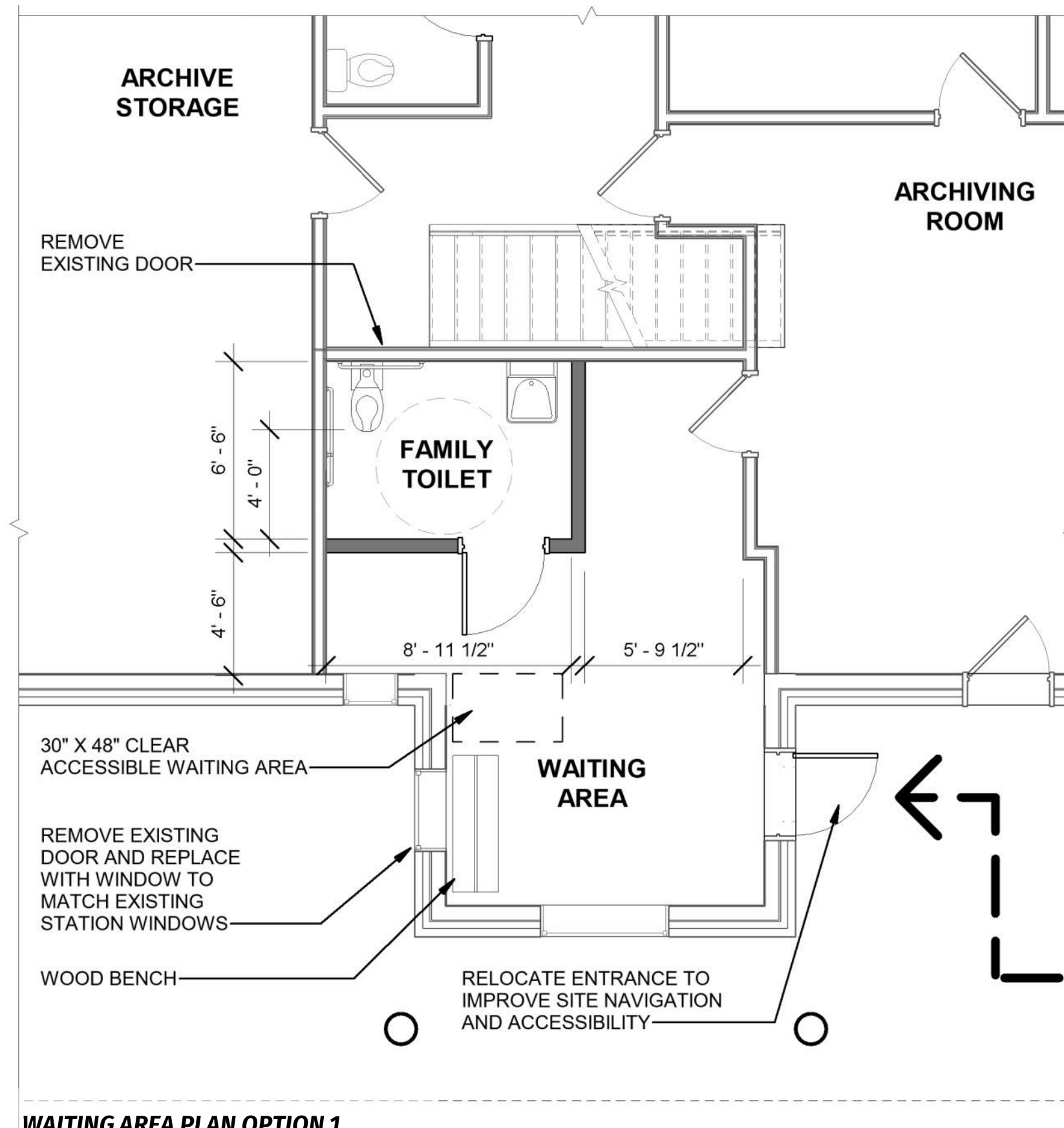
WAITING AREA PLAN OPTION 1
