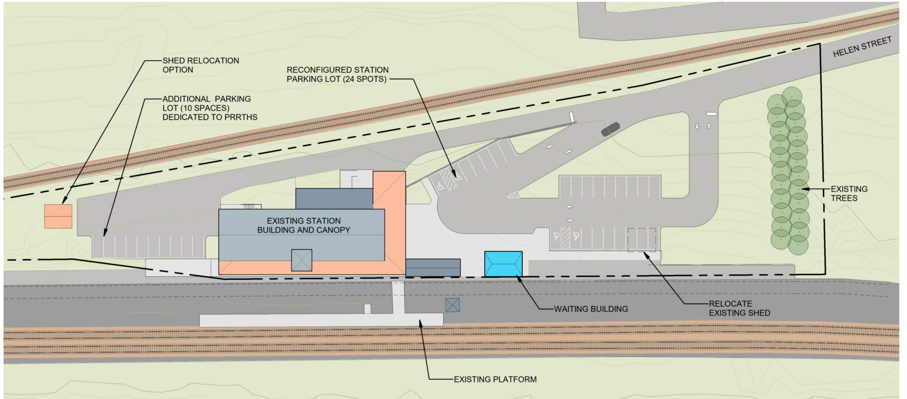
SITE PLAN OPTION 1 – WITHOUT BUS STOP
