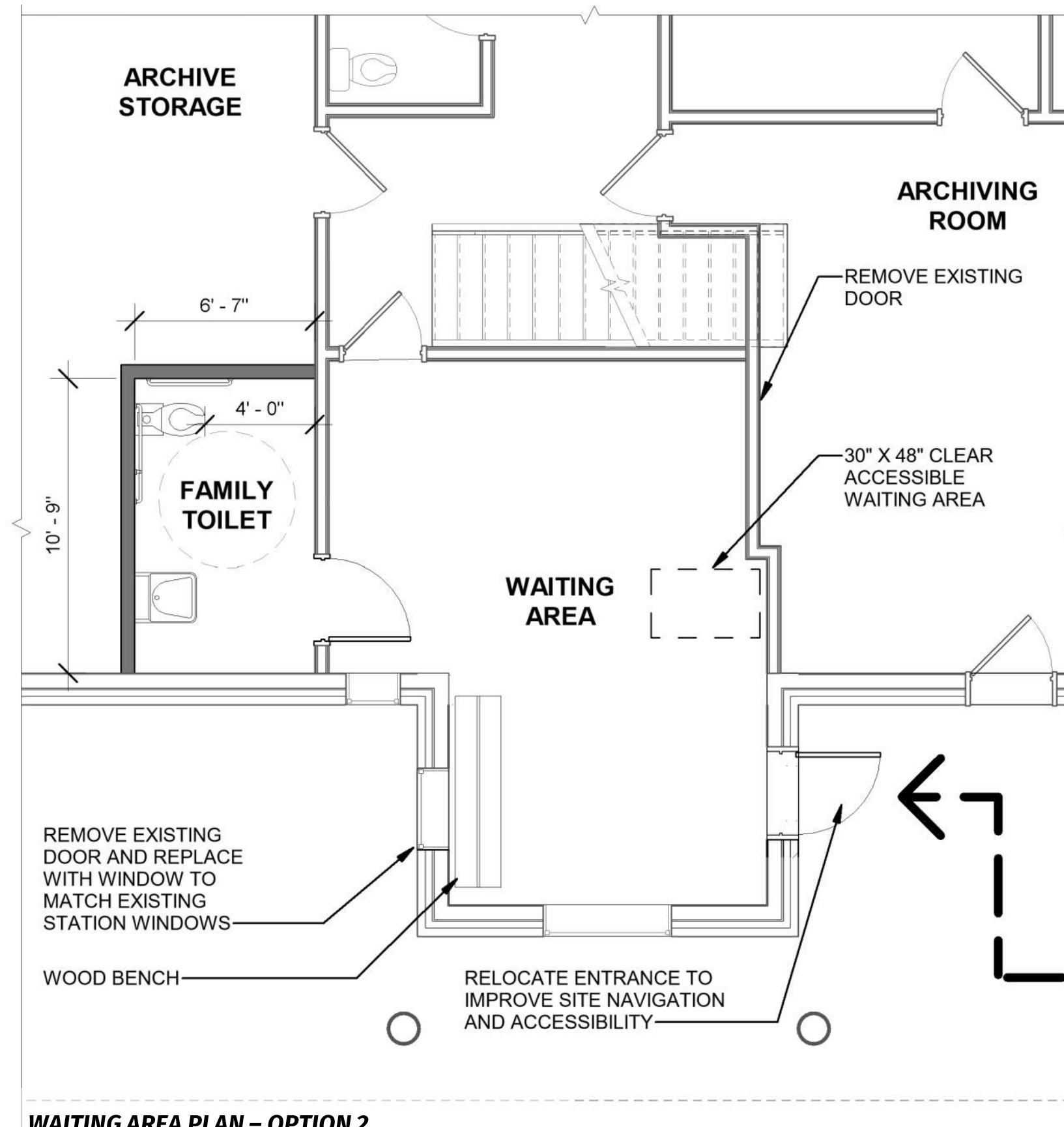
WAITING AREA PLAN – OPTION 2
