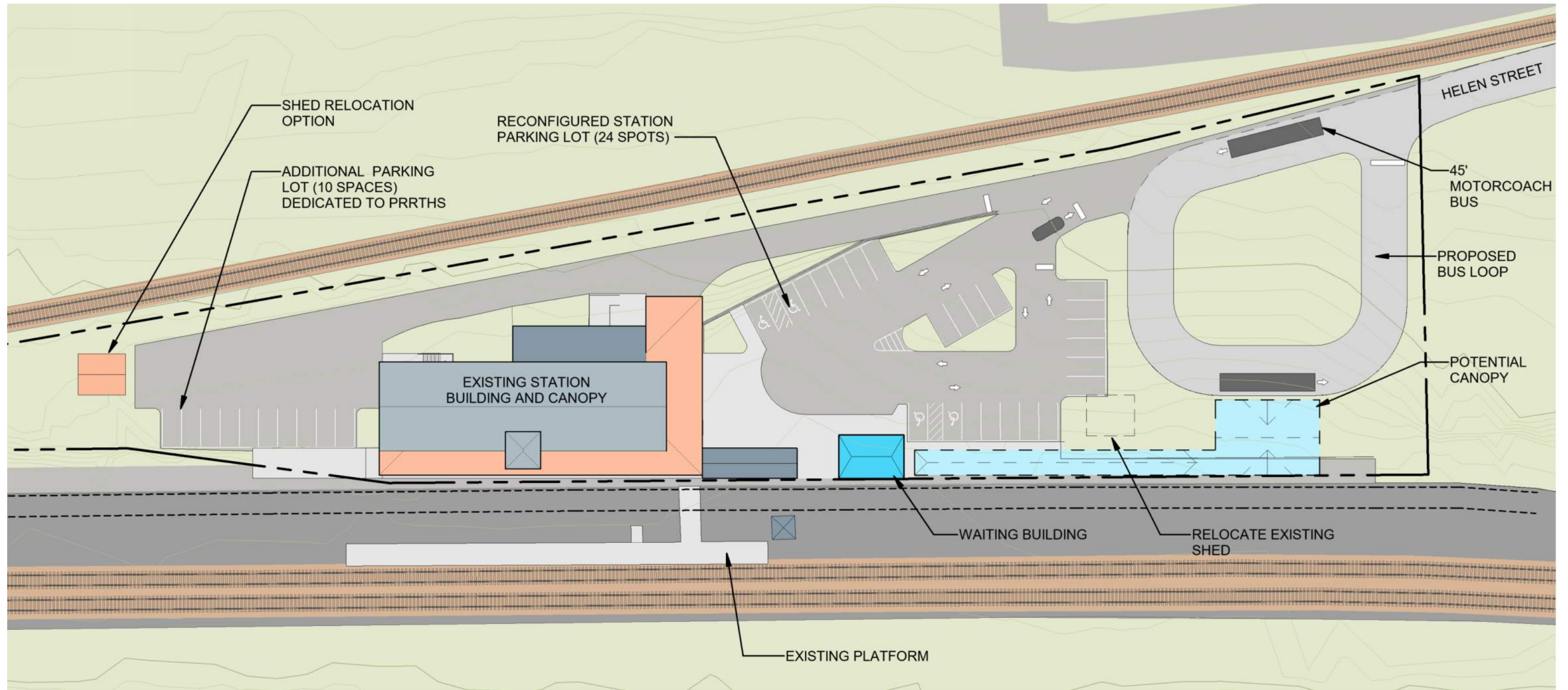
SITE PLAN OPTION 2 – WITH BUS STOP
